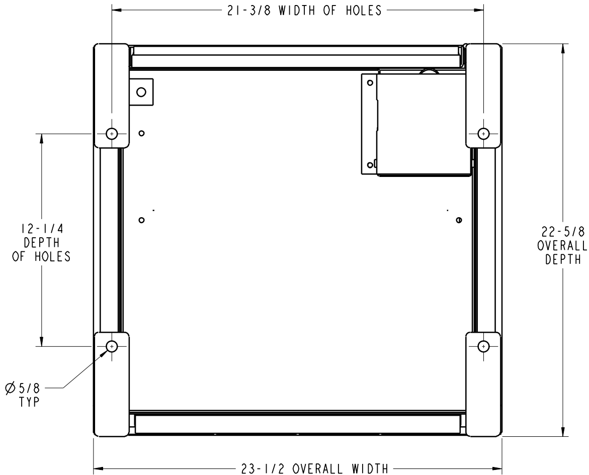
BOTTOM VIEW FOOTPRINT OF CONTAINER & HOLE LOCATIONS
